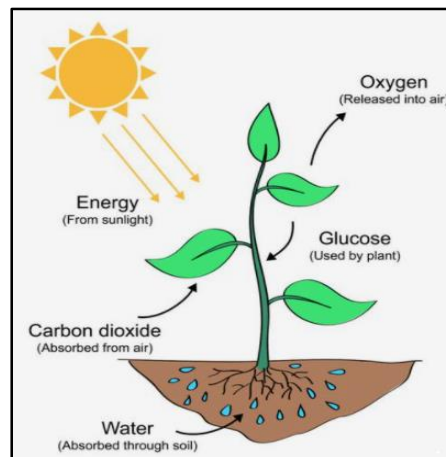
b) Photosynthesis
